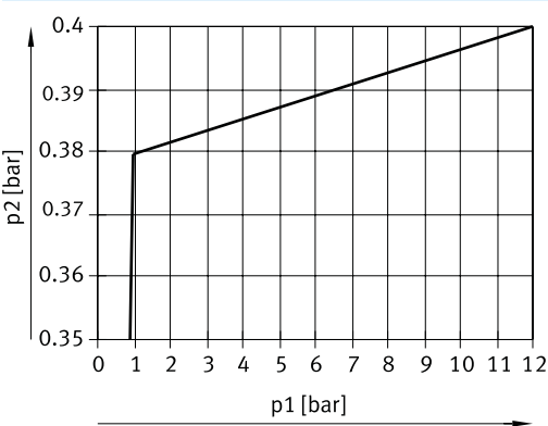
Output pressure p_2 as a function of operating pressure p_1 (size 50, primary pressure dependence q_n = 35 \text{ l/min} )
