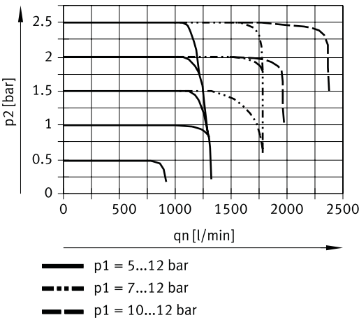
Standard flow rate q_n as a function of output pressure p_2 – LRP/LRPS-1/4-2.5
